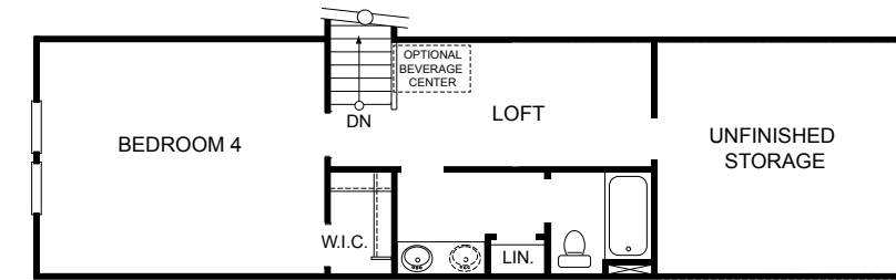
STANDARD INCLUDES BEDROOM #4, LOFT, FULL BATH AND UNFINISHED STORAGE
